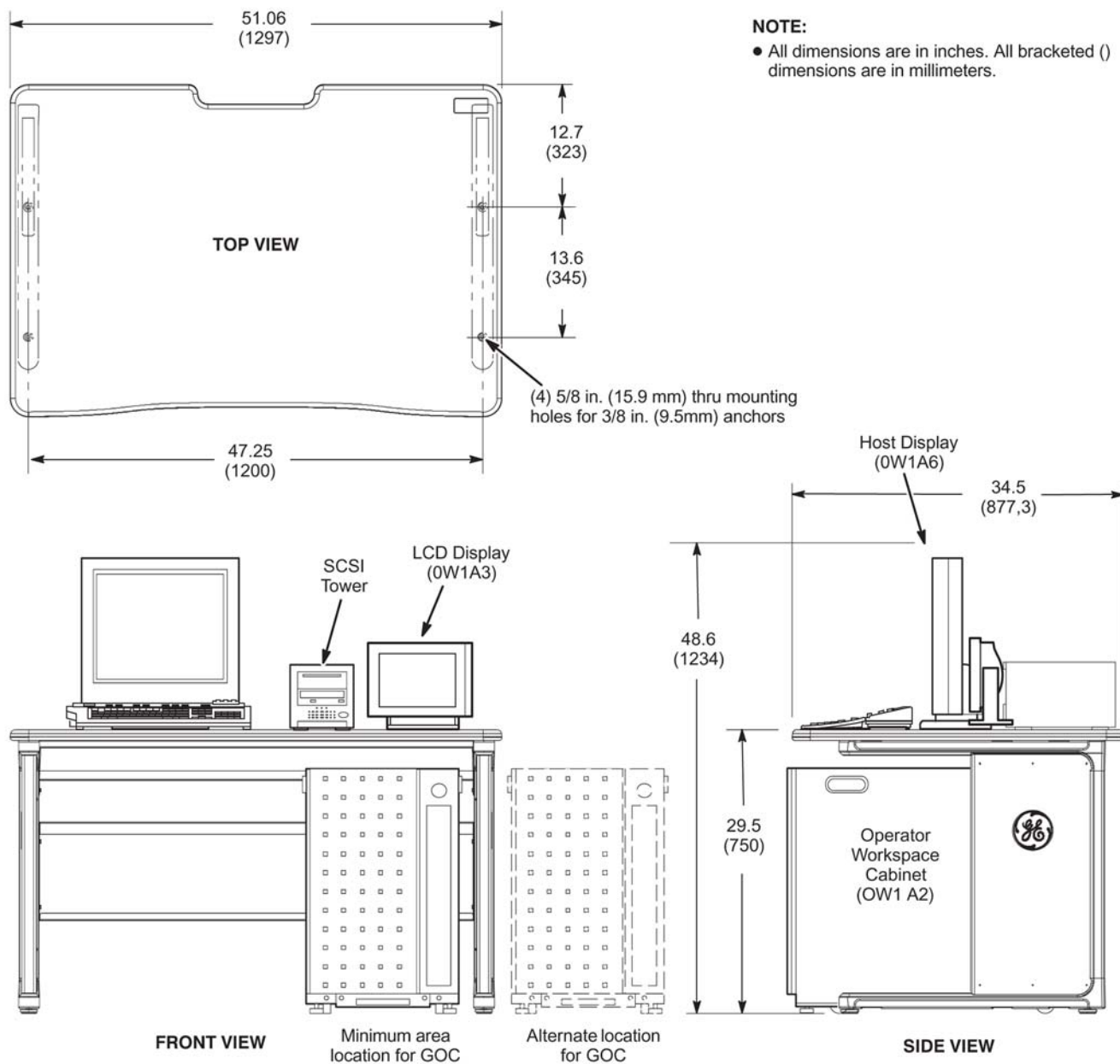
Illustration 3-16: Operator Workspace (OW1) Overall Dimensions
