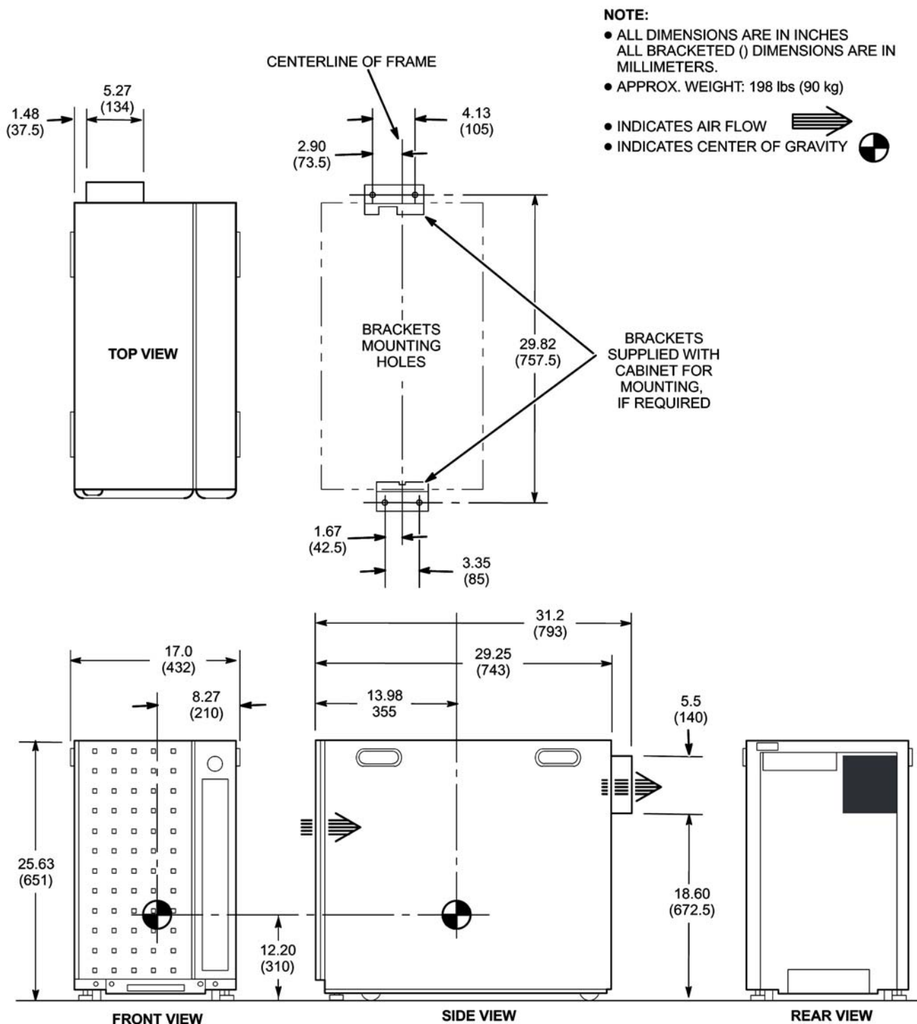
Illustration 3-17: GOC Computer Cabinet (OW1 A2)
