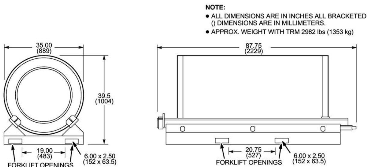
Illustration 3-11: Replacement TRM Gradient Coil Assembly & Cradle
