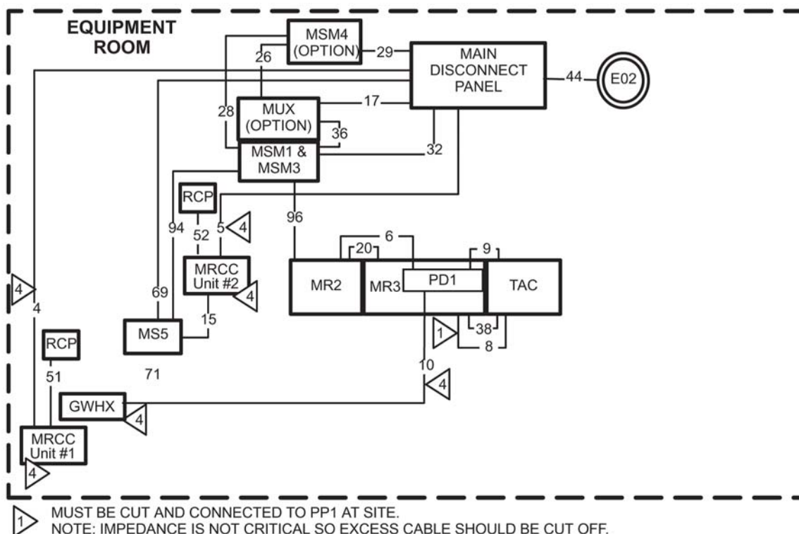
Illustration 7-15: System L3 Interconnects Diagram
