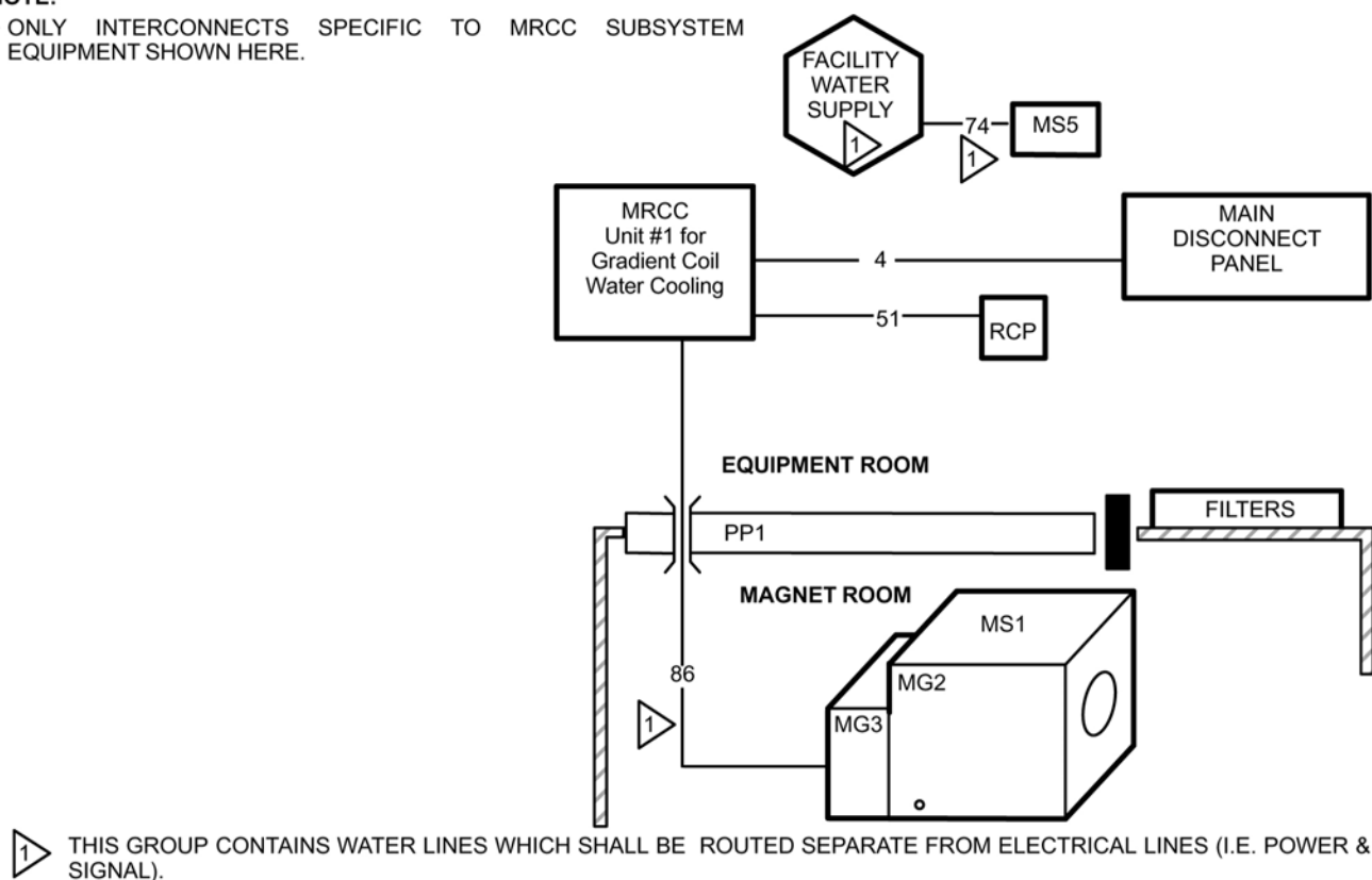
Illustration 7-28: 1 MRCC Unit Located Indoor & RCP Subsystem Group Interconnect Diagram
