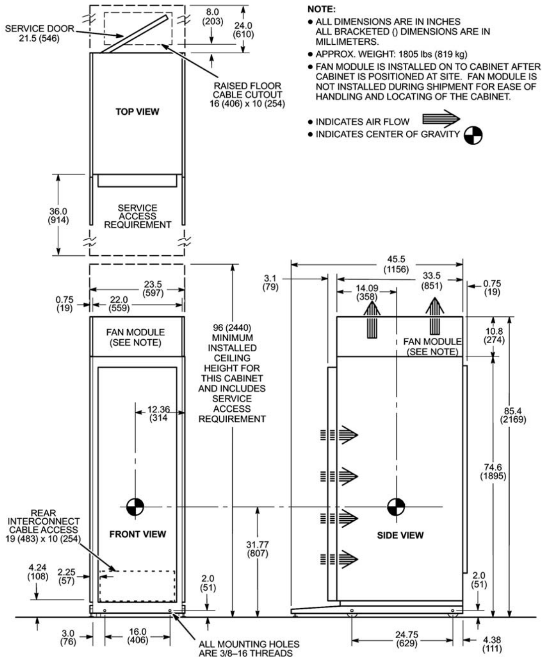
Illustration 3-37: HFD/PDU Cabinet (MR3)
