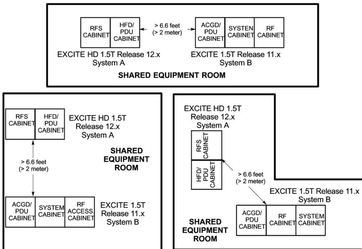
Illustration 3-3: Multiple Signa EXCITE HD 1.5T (Release 12.x) & Signa EXCITE 1.5T (Release 11.x) Systems Electronics Cabinets Spacing
