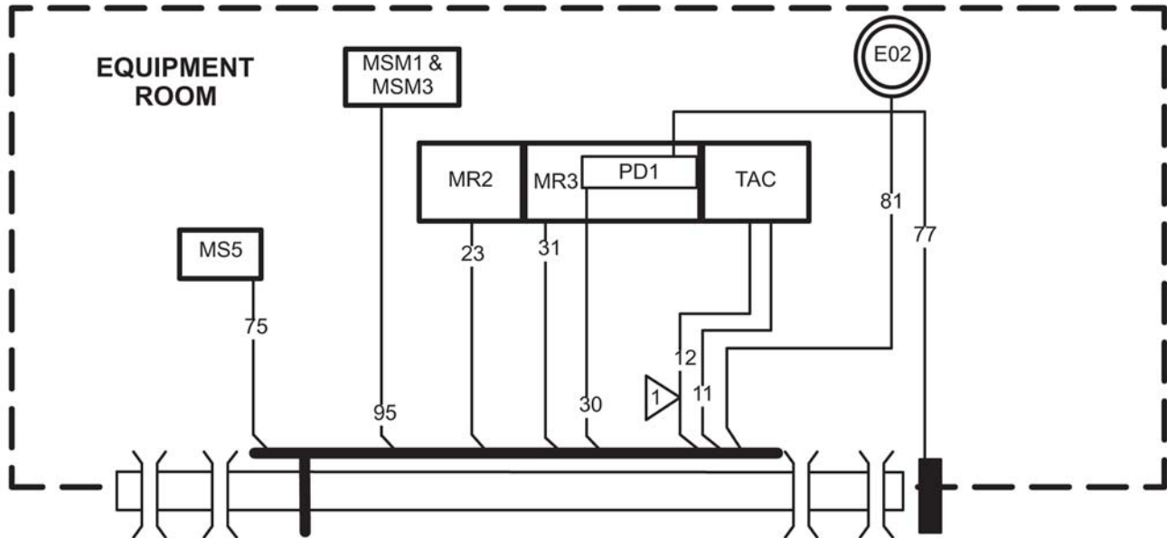
Illustration 7-11: System L2 Interconnects Diagram
