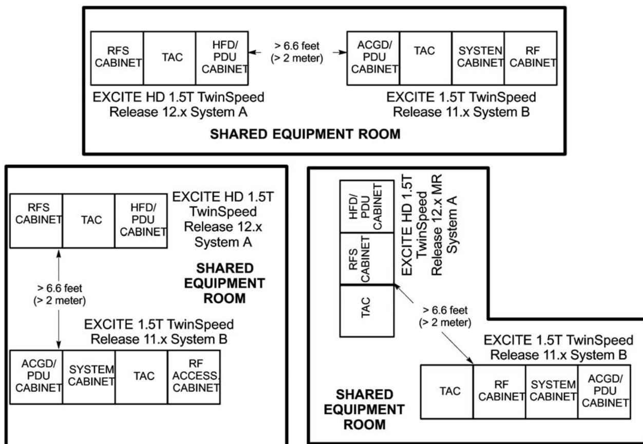
Illustration 3-5: Multiple Signa EXCITE HD 1.5T TwinSpeed (Release 12.x) & Signa EXCITE 1.5T TwinSpeed (Release 11.x) Systems Electronics Cabinets Spacing
