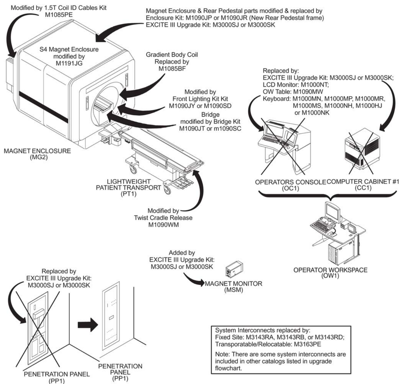
Illustration 2-24: Signa Advantage 5.x Existing Hardware Replaced Or Modified & New Equipment Added
