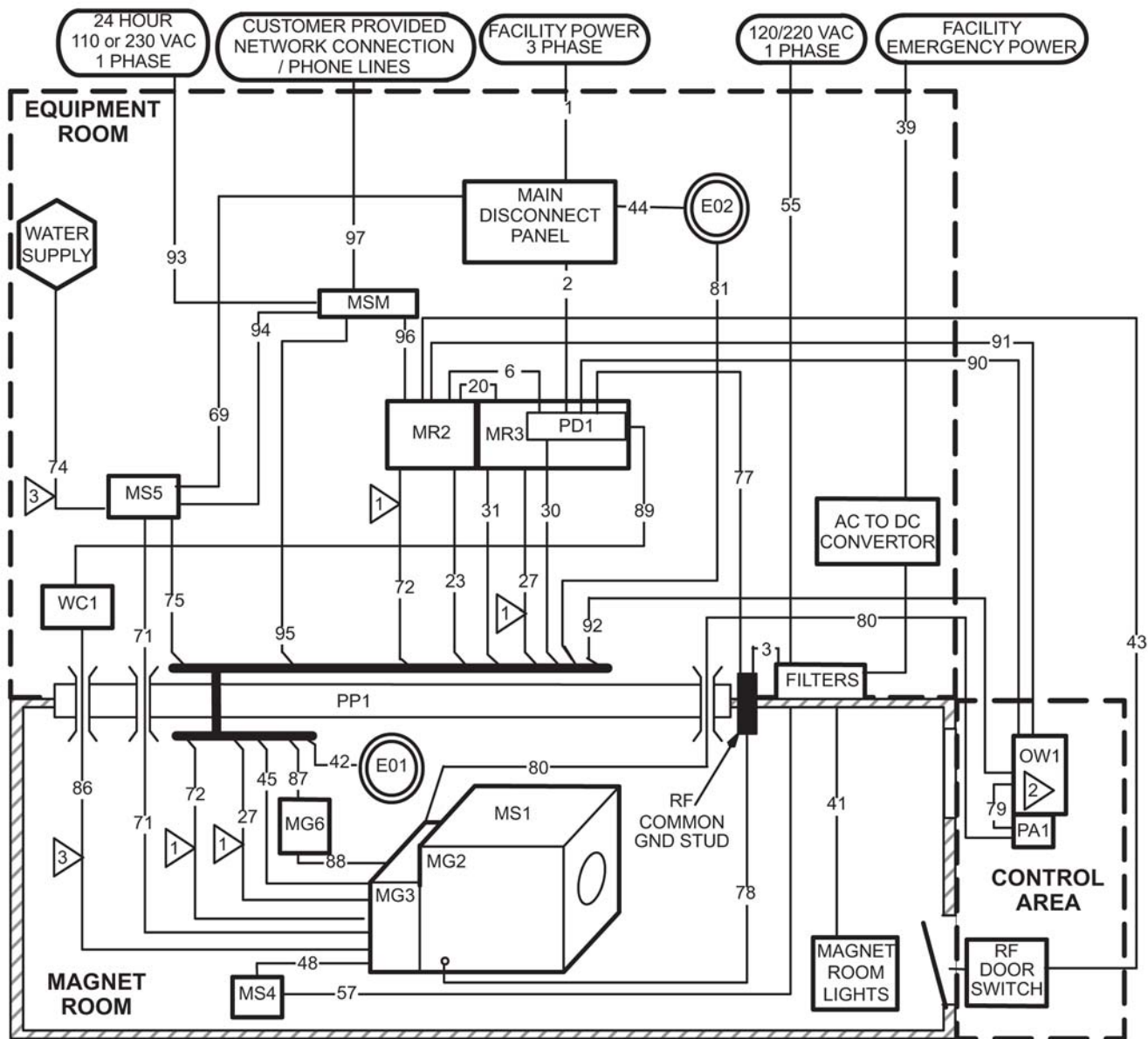
Illustration 7-21: Signa EXCITE HD 1.5T System Group Interconnect Diagram
