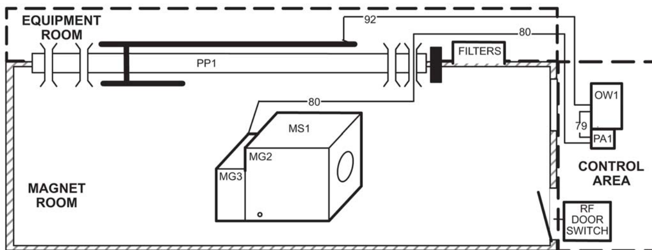
Illustration 7-16: System L4 Interconnects Diagram
