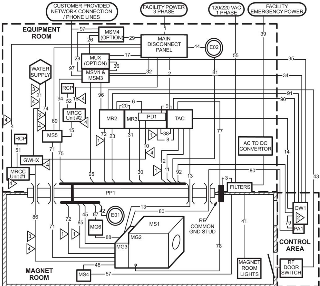
Illustration 7-22: Signa EXCITE HD 1.5T TwinSpeed System Group Interconnect Diagram
