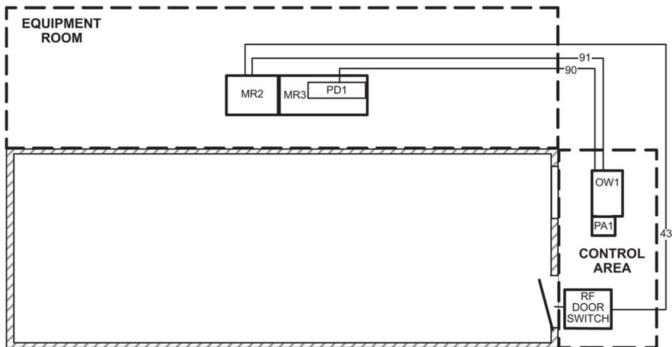
Illustration 7-17: System L5 Interconnects Diagram
