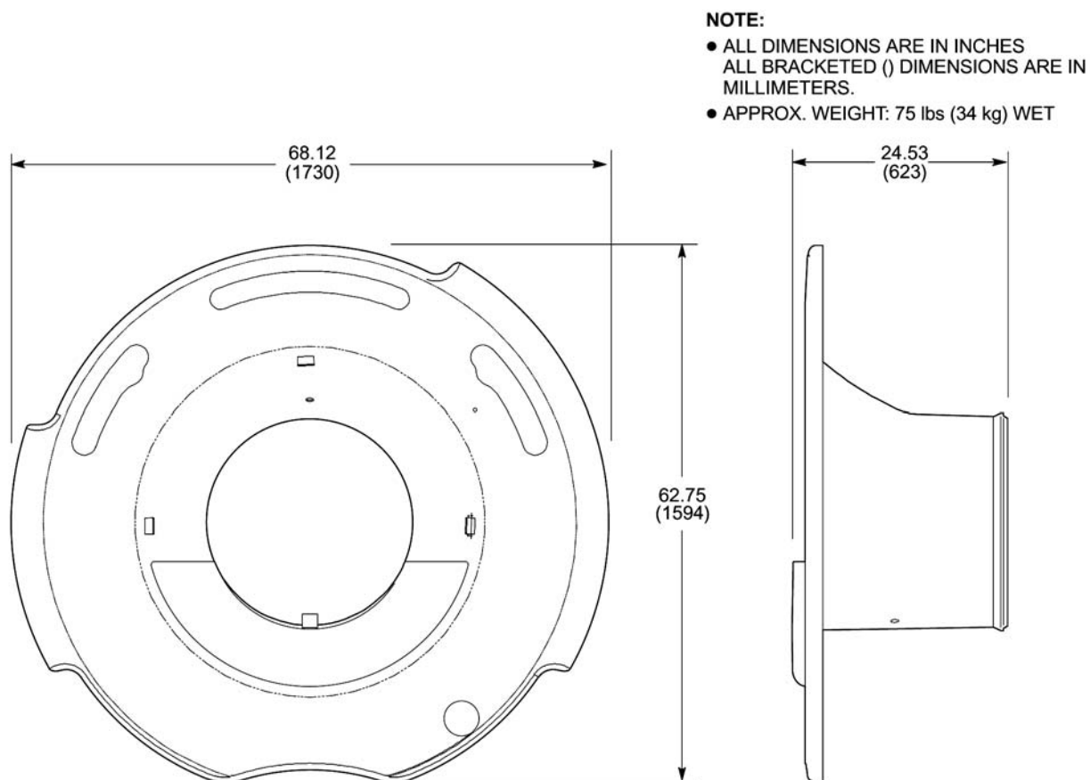
Illustration 3-44: Horizon Enclosure Upgrade Front Endbell
