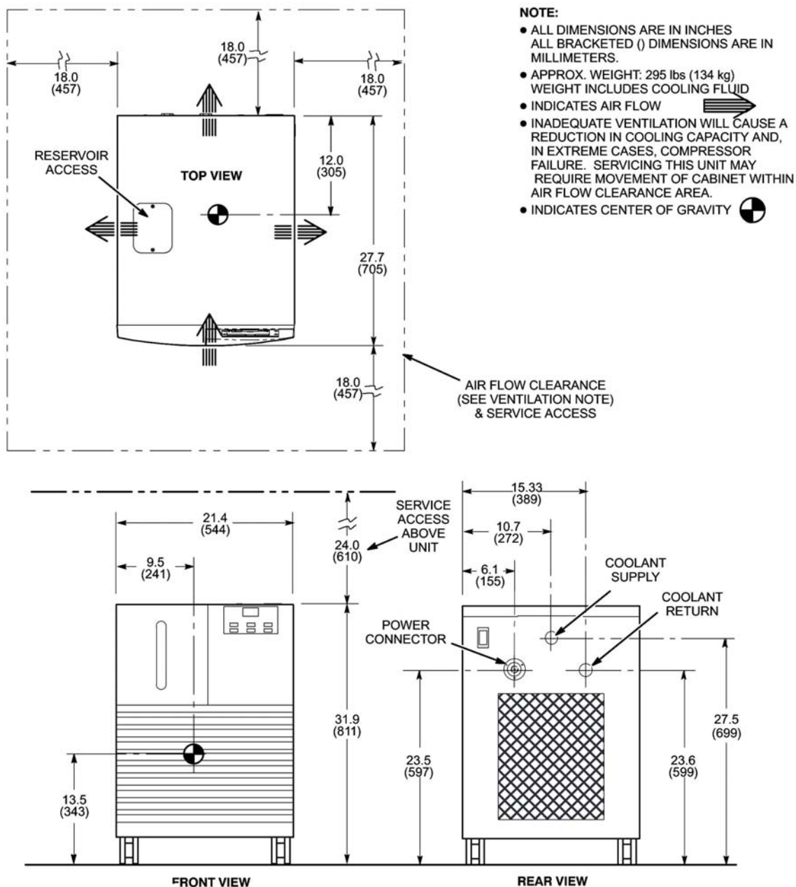
Illustration 3-24: Water Chiller (WC1) For BRM Gradient Coil Cooling Water
