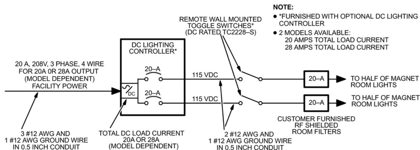
Illustration 6-6: Variable DC Lighting Controller (Facility Option) Wiring Diagram
