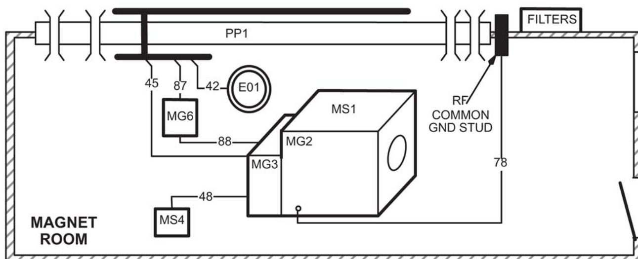
Illustration 7-8: System L1 Interconnects Diagram
