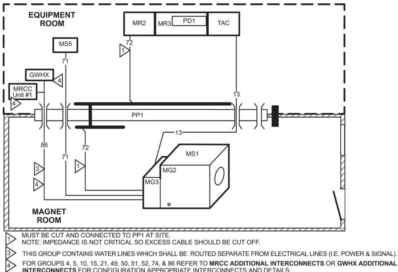
Illustration 7-13: System L1/L2 Interconnects Diagram
