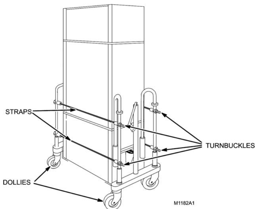
Illustration 3-14: Full-Size PDU Shipping Dollies
