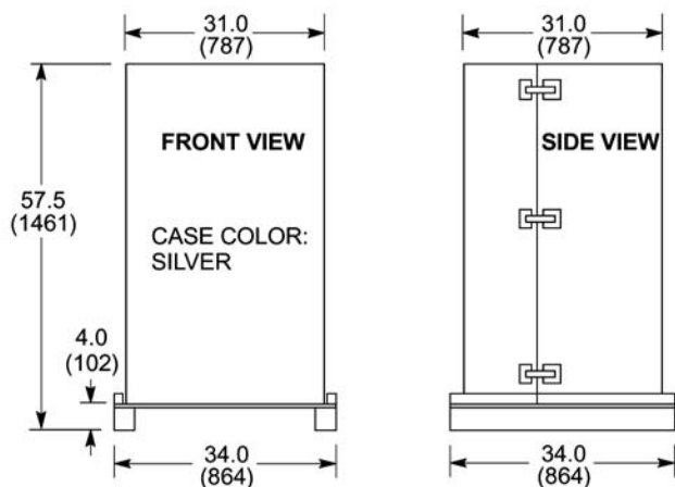
Illustration 3-38: TwinSpeed RF Coil In Shipping Case
