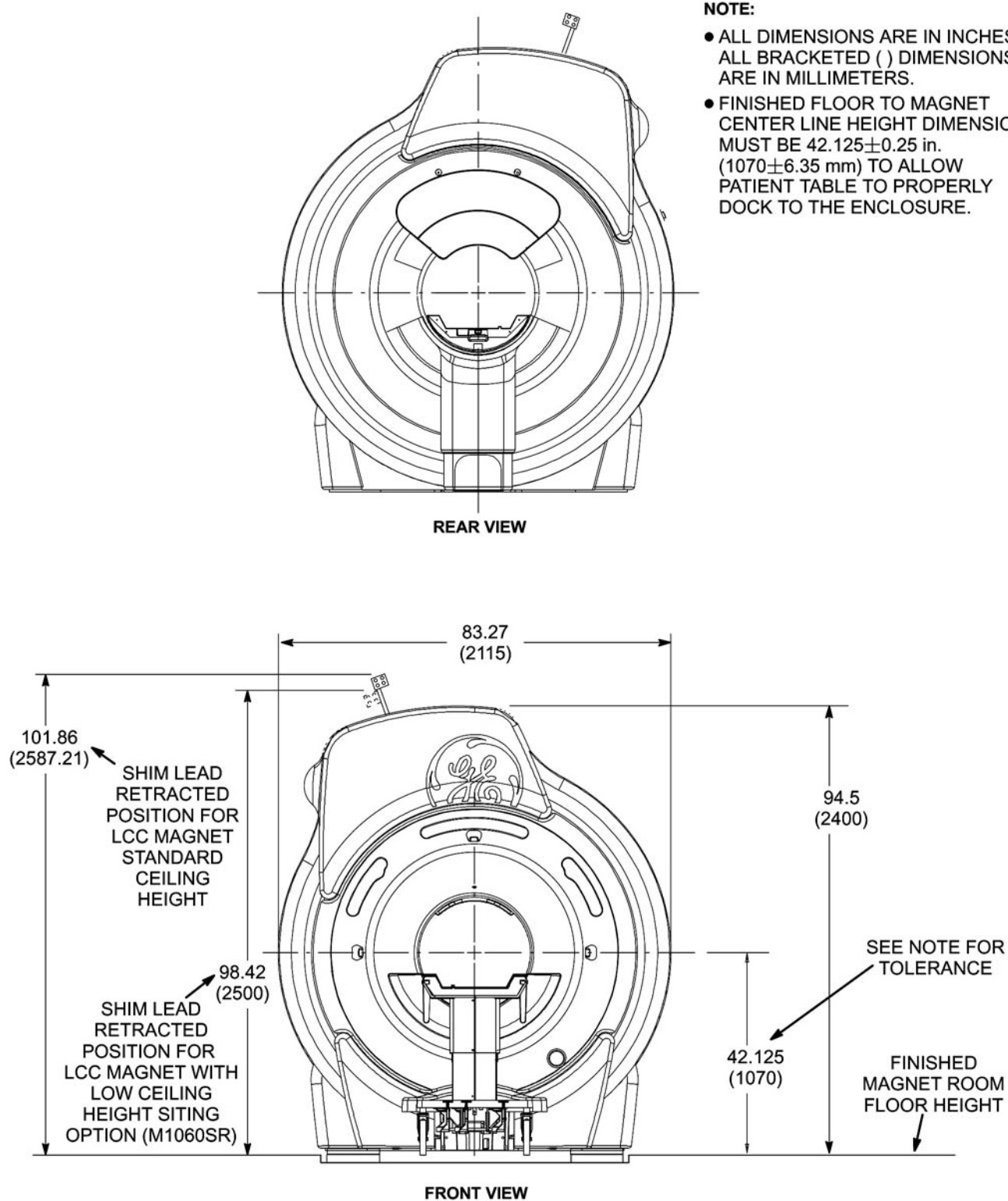
Illustration 3-45: Magnet (with TRM) Enclosure Front And Rear Views
