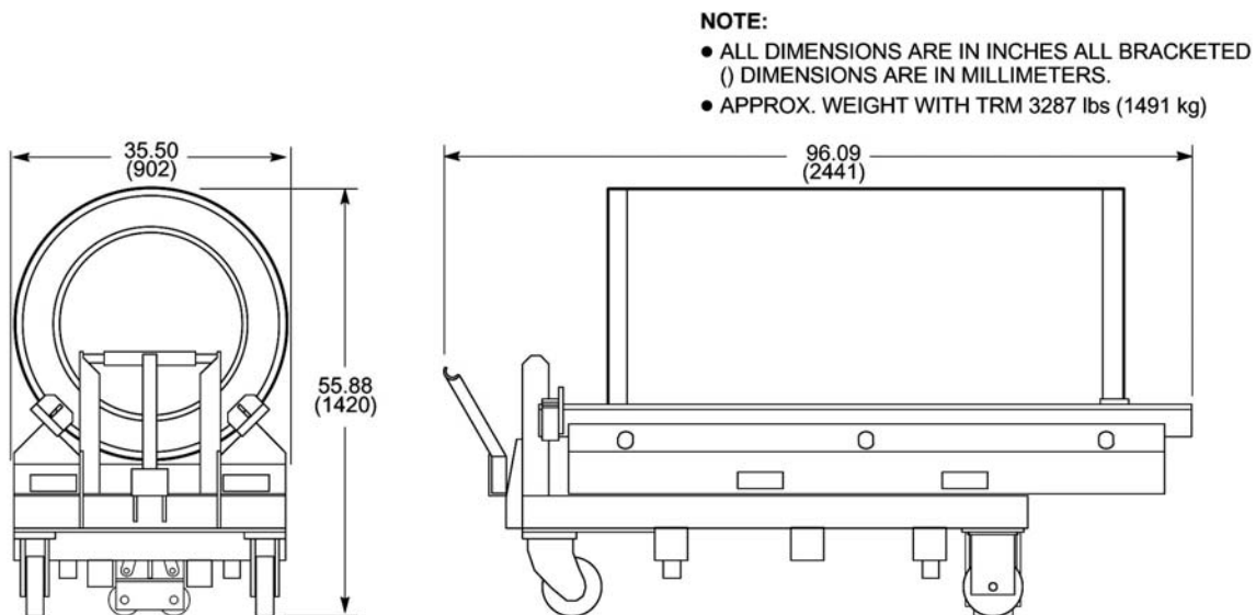
Illustration 3-10: Short Room Replacement BRM Gradient Coil Assembly & Cradle On Cart
