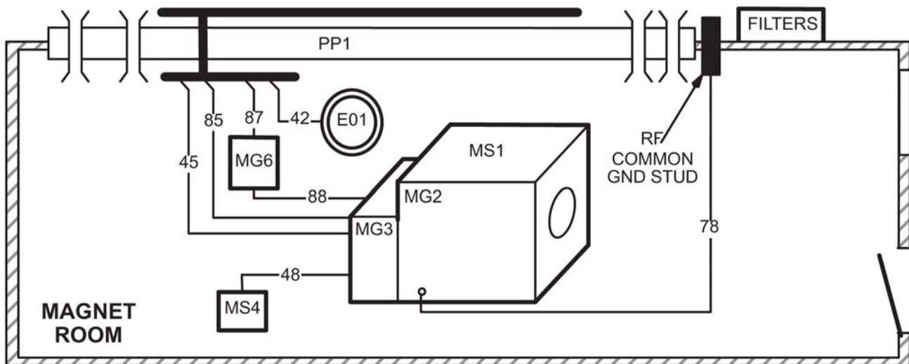
Illustration 7-9: System L1 Interconnects Diagram
