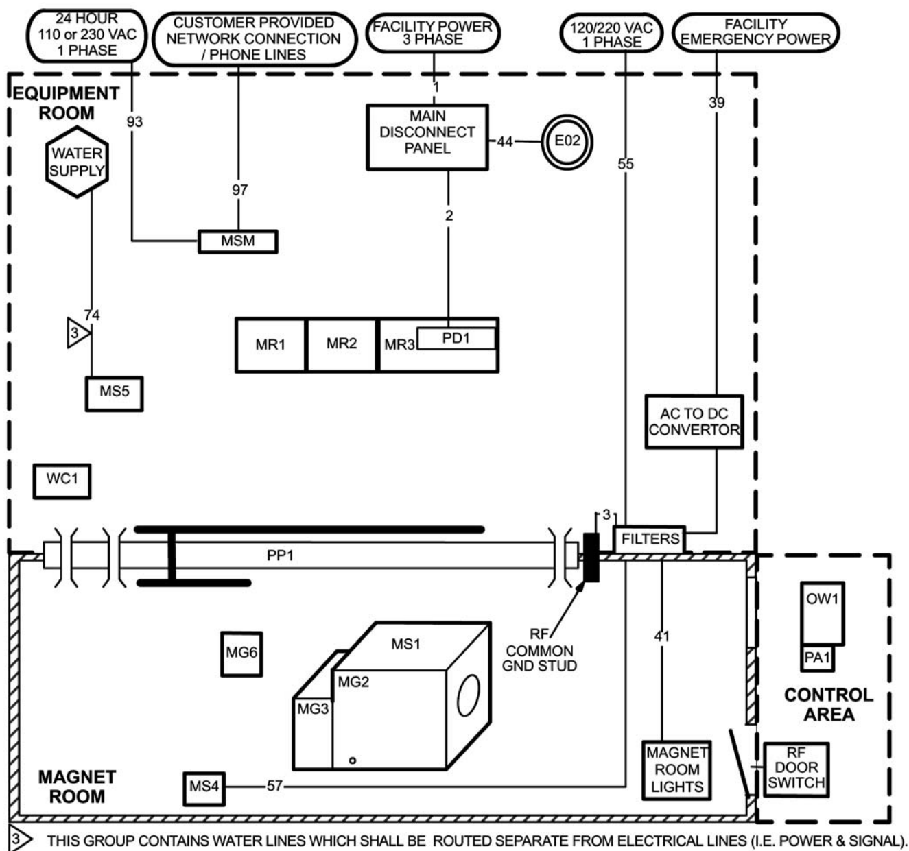
Illustration 7-19: System Customer Supplied Interconnects Diagram
