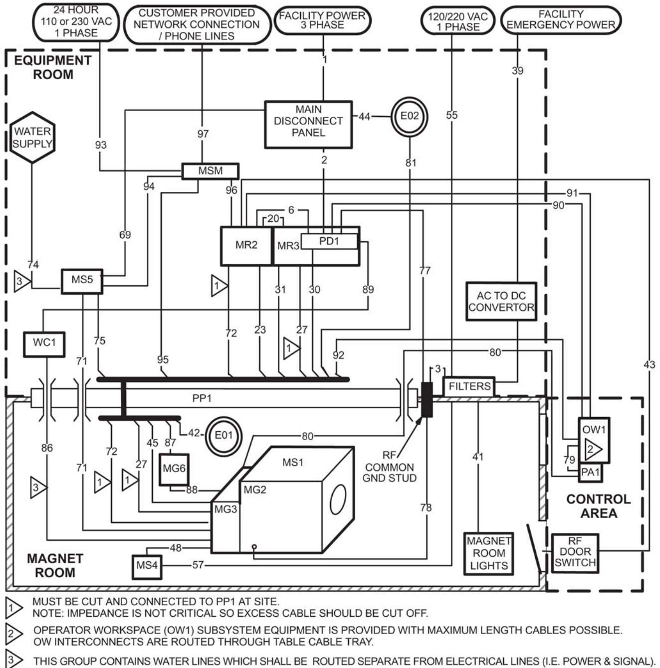
Illustration 7-6: Signa EXCITE HD 1.5T System Group Interconnect Diagram
