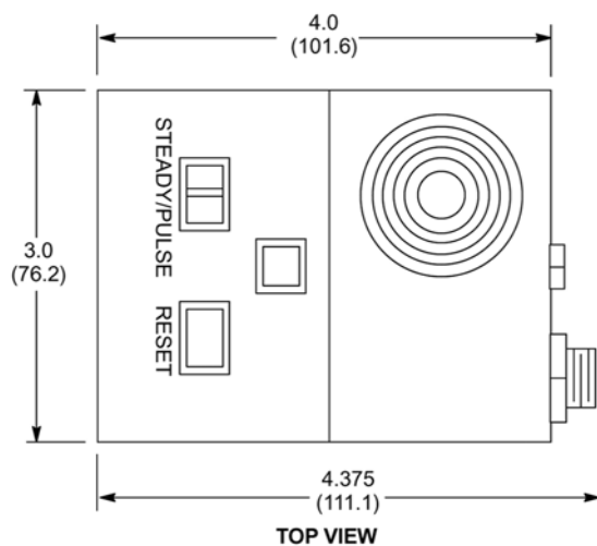
Illustration 3-21: Pneumatic Patient Alert Control Box (PA1)
