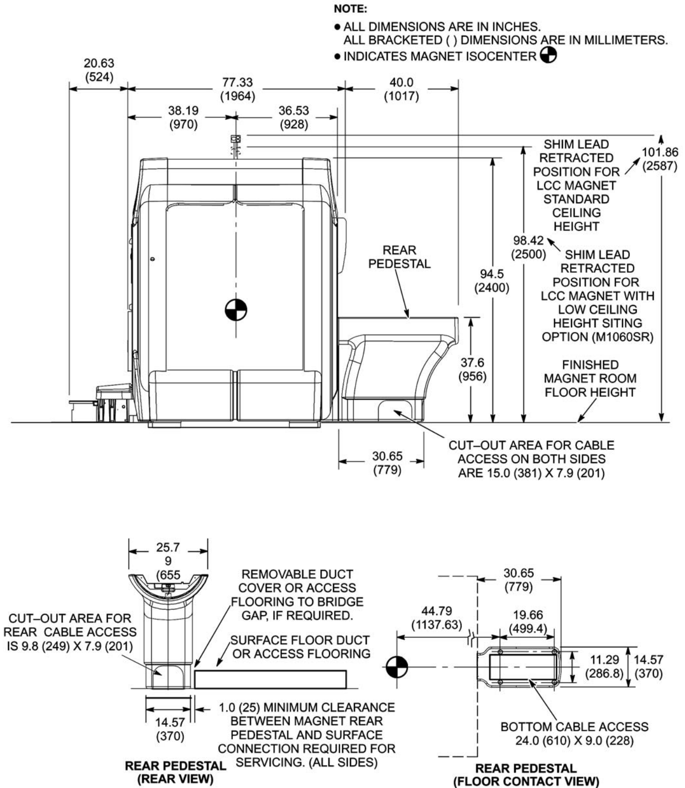
Illustration 3-46: Magnet Enclosure Cable Access
