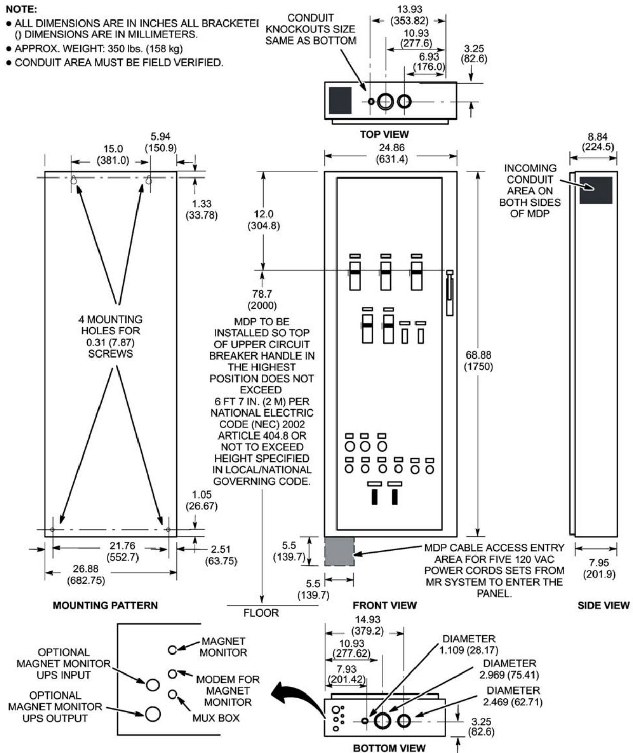
Illustration 3-49: Signa TwinSpeed Main Disconnect Panel (MDP) M3088TM
