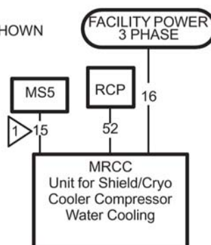
Illustration 7-24: MRCC Units Located Indoor & RCP Subsystem Group Interconnect Diagram
