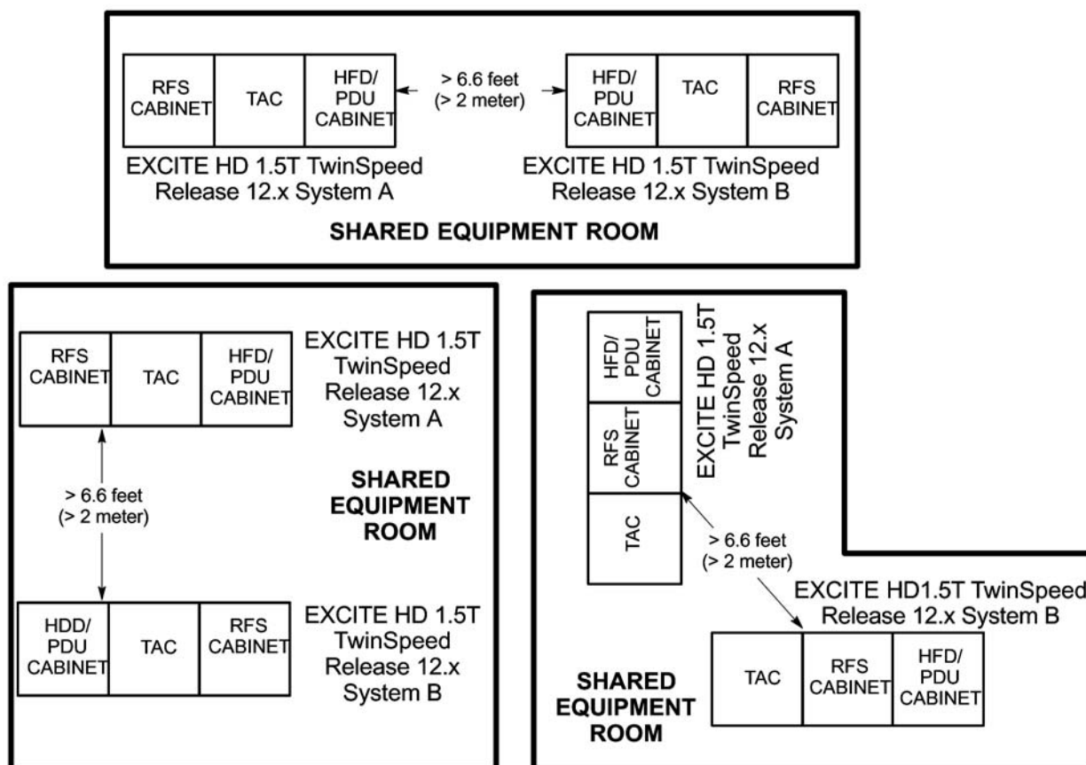
Illustration 3-4: Multiple Signa EXCITE HD 1.5T TwinSpeed (Release 12.x) Systems Electronics Cabinets Spacing
