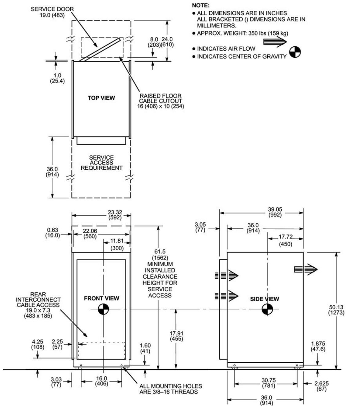
Illustration 3-51: 1.5T MNS Cabinet (MR10) for 2 KW MNS Option
