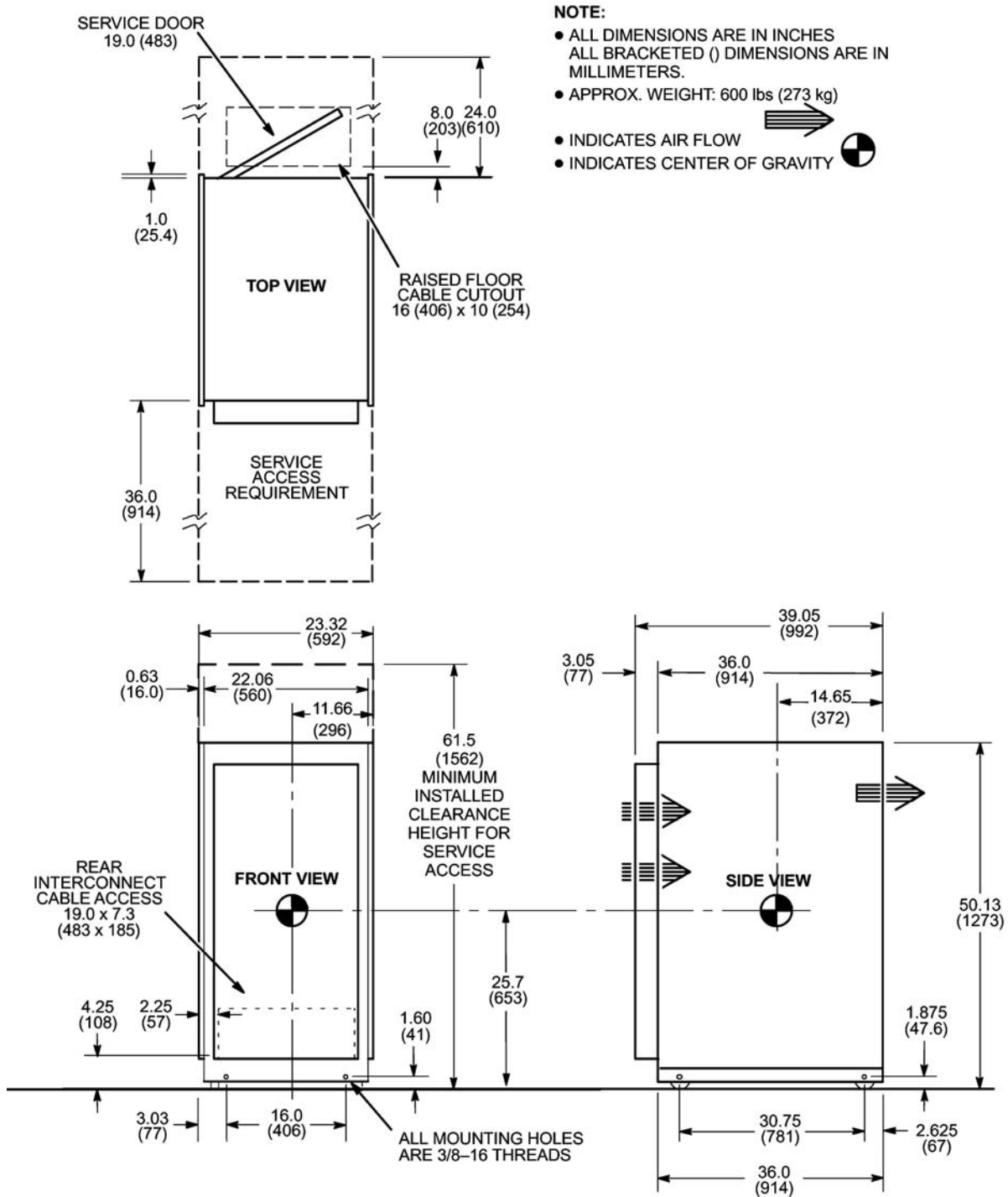
Illustration 3-40: 1.5T Twin Accessory Cabinet (TAC)
