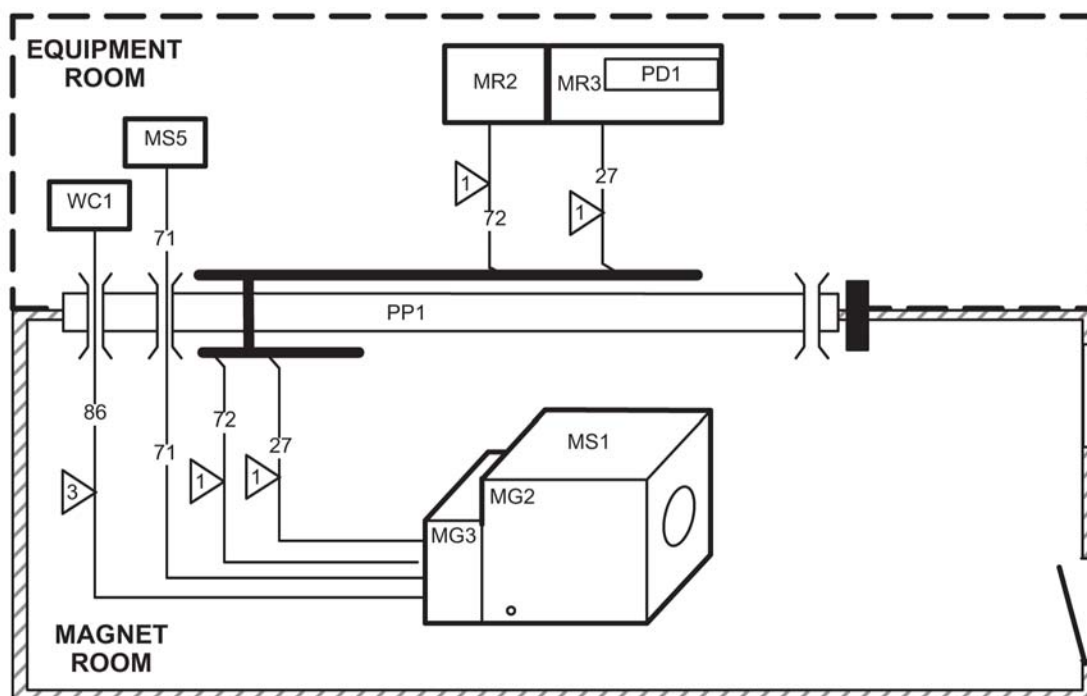
Illustration 7-12: System L1/L2 Interconnects Diagram
