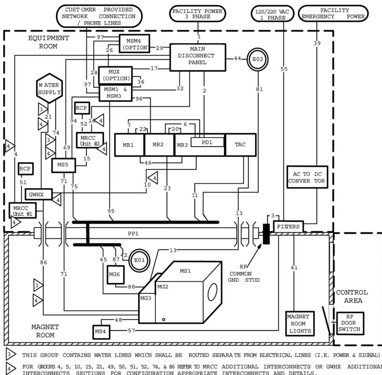
Illustration 7-5: Release 11.x To Release 12.x TwinSpeed Upgrades System Group Interconnect Diagram
