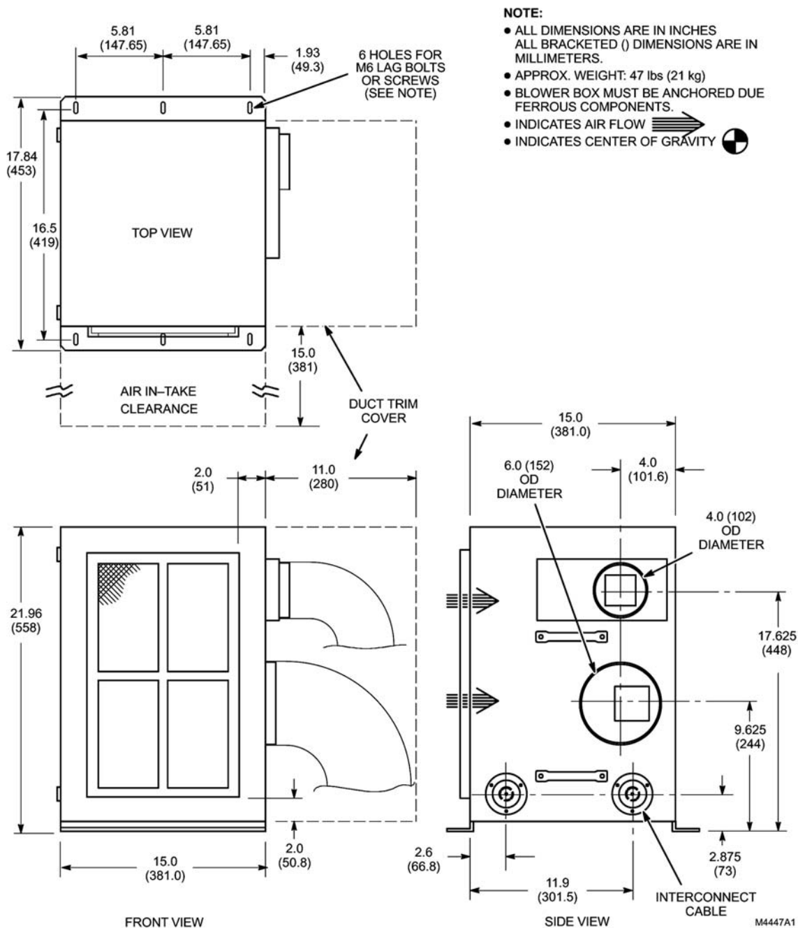
Illustration 3-33: Blower Box (MG6)
