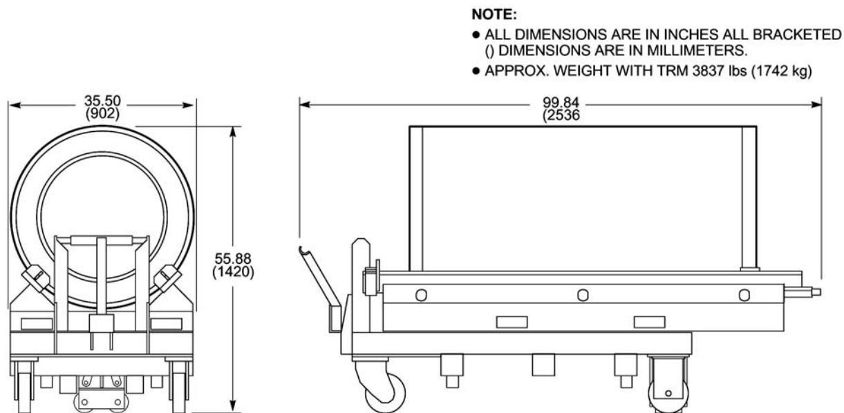
Illustration 3-12: Short Room Replacement TRM Gradient Coil Assembly & Cradle On Cart
