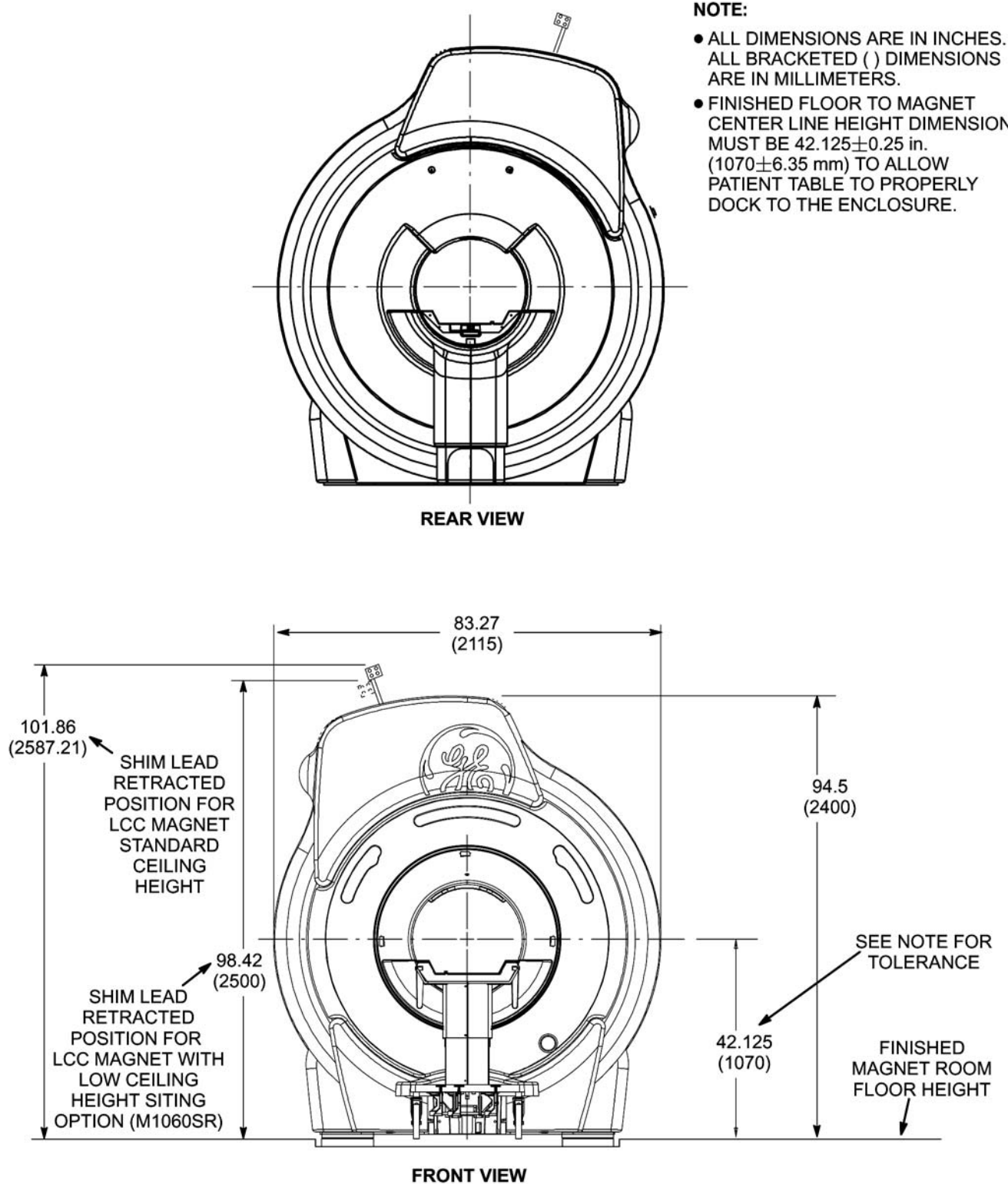
Illustration 3-22: Magnet (with BRM) Enclosure Front And Rear Views
