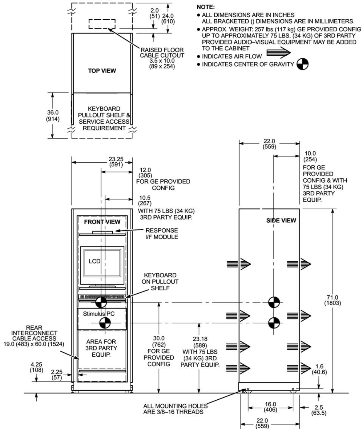
Illustration 3-52: Brainwave HW Lite Cabinet
