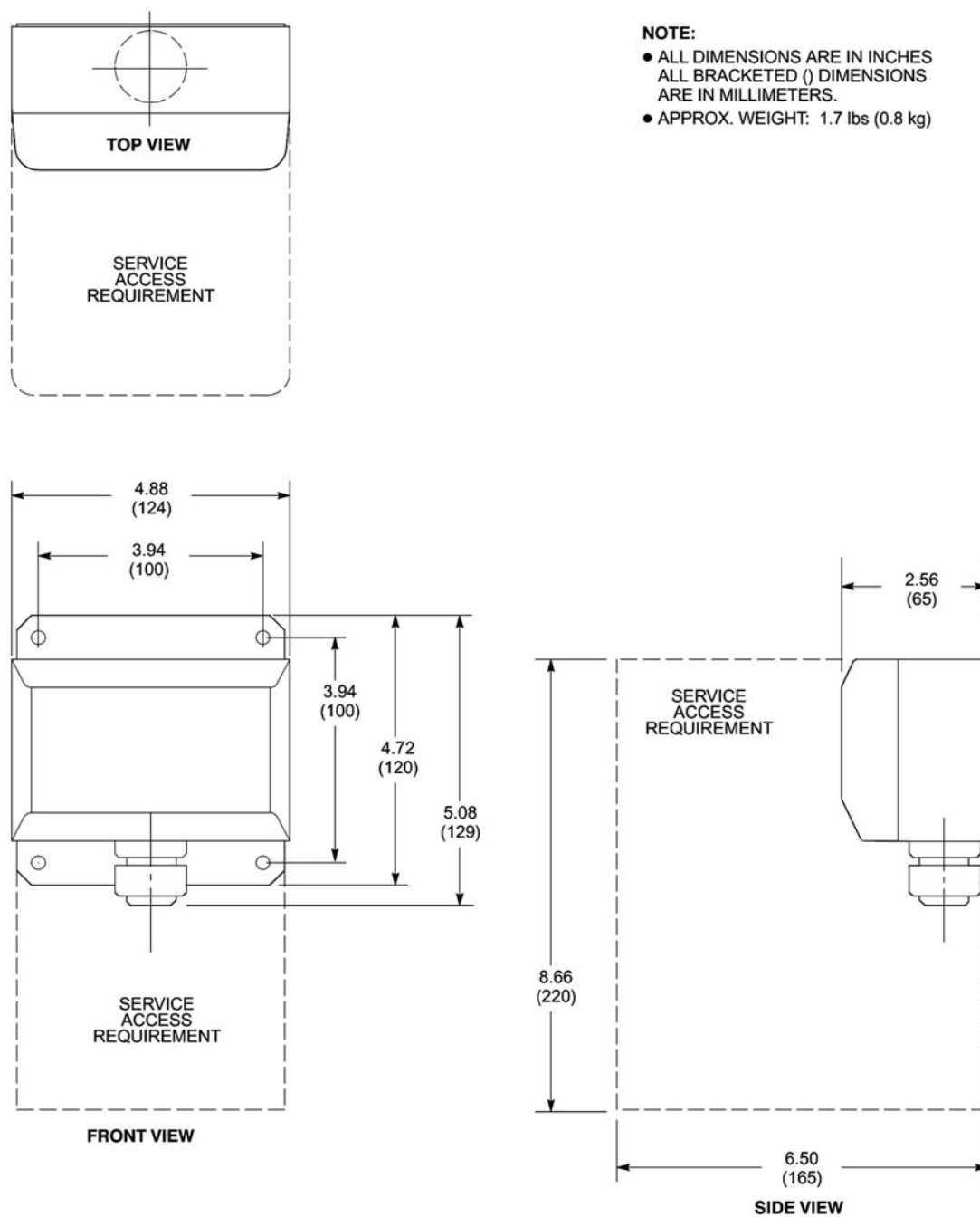
Illustration 3-48: Remote Control Panel (RCP) For MRCC
