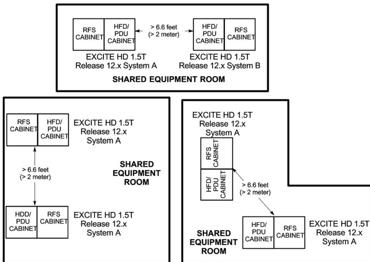
Illustration 3-2: Multiple Signa EXCITE HD 1.5T (Release 12.x) Systems Electronics Cabinets Spacing
