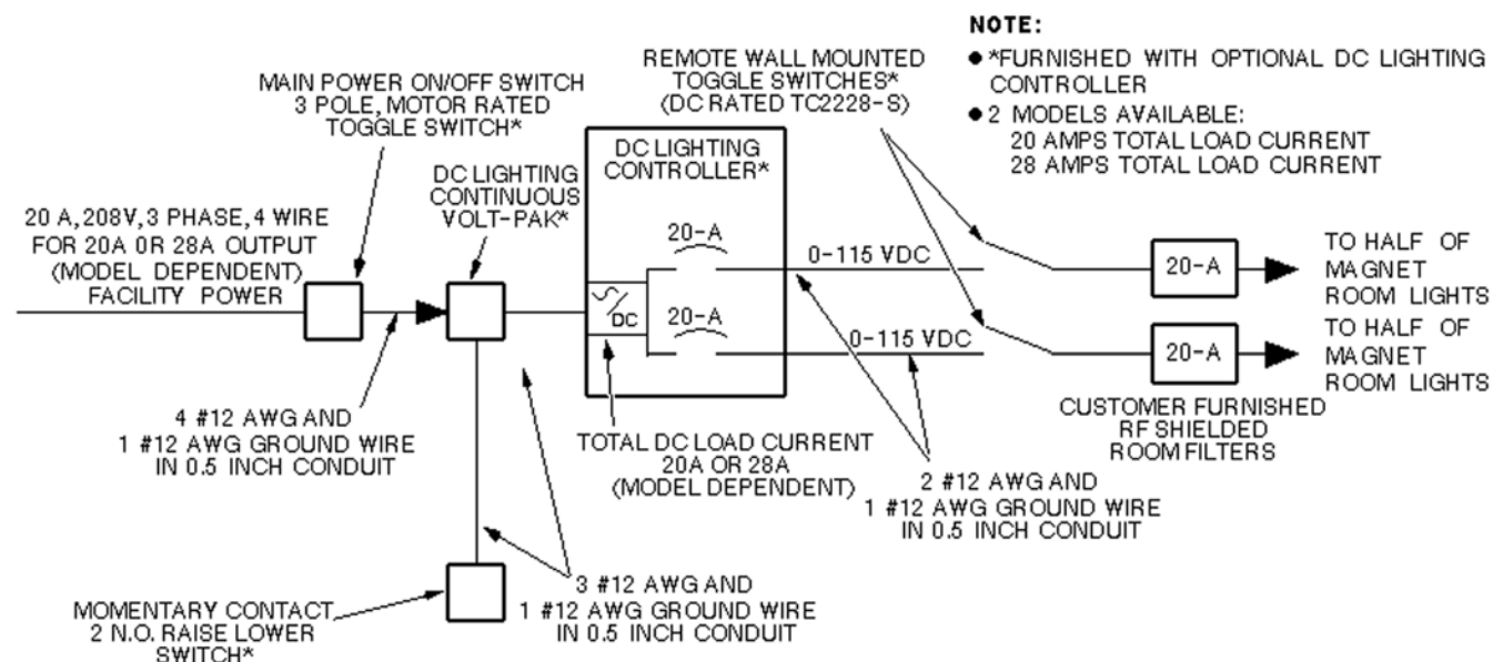
Illustration 6-6: Variable DC Lighting Controller (Facility Option) Wiring Diagram
