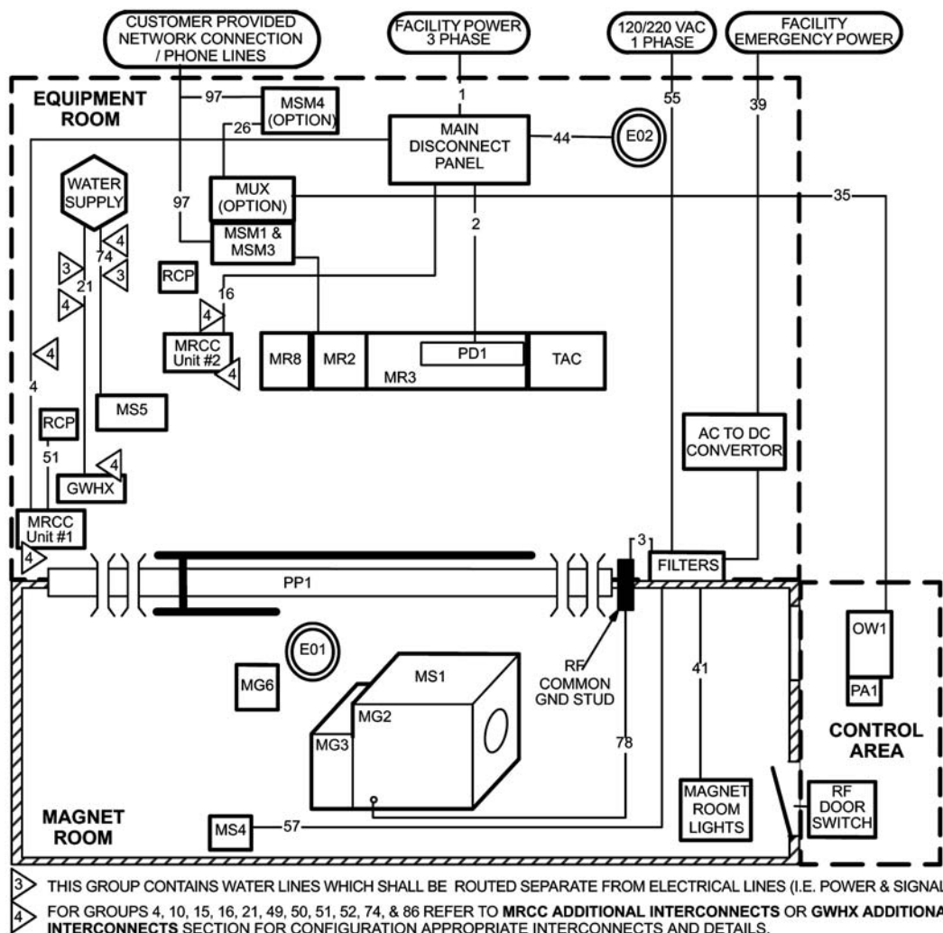
Illustration 7-20: System Customer Supplied Interconnects Diagram
