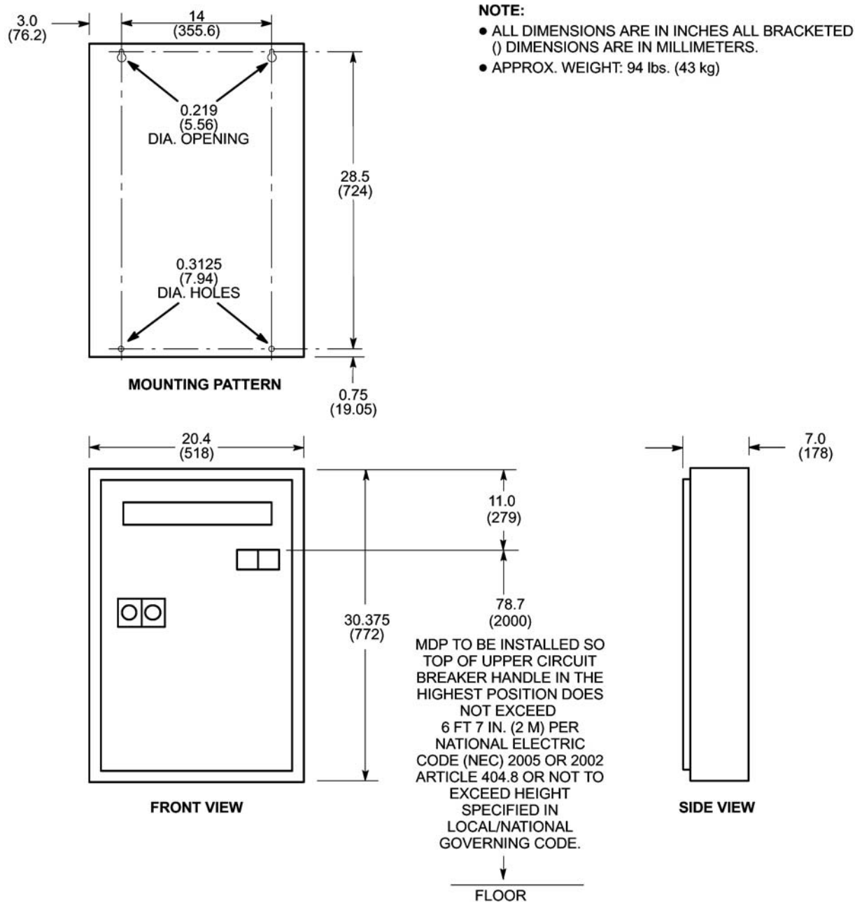
Illustration 3-50: Signa Main Disconnect Panel E4502SP Option
