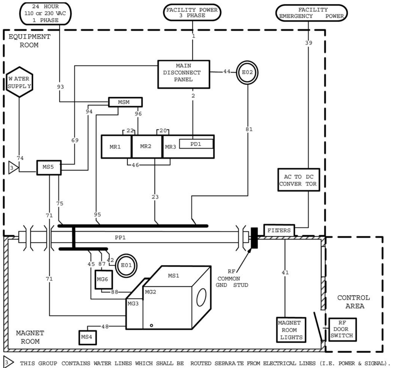
Illustration 7-4: Release 11.x To Release 12.x Upgrades System Group Interconnect Diagram
