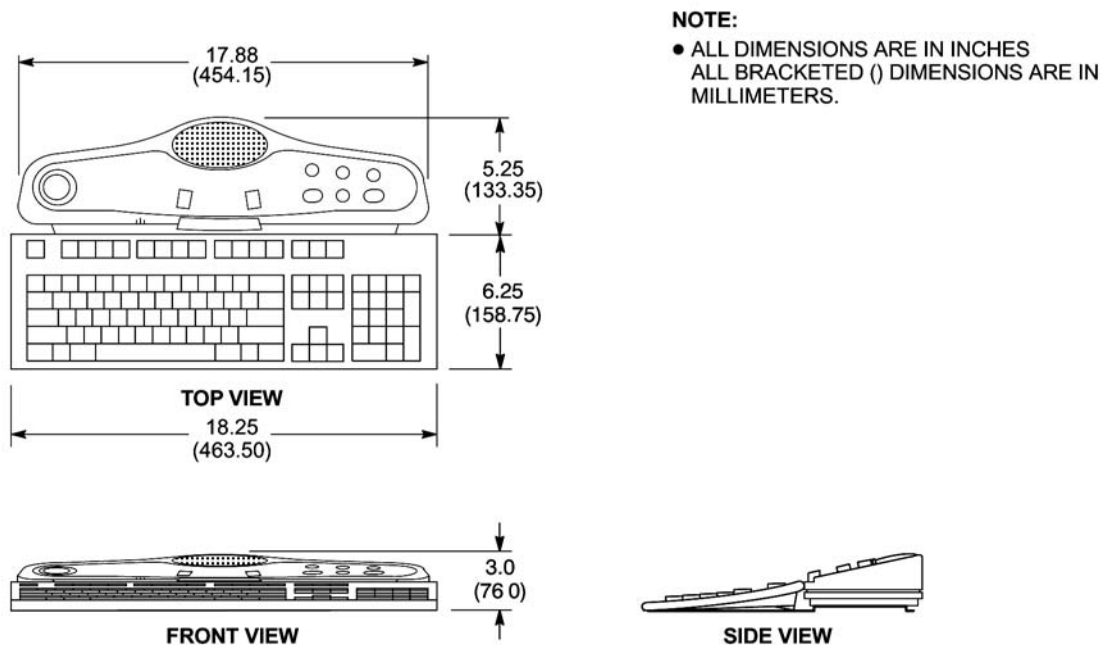
Illustration 3-20: Operator Workspace Components Position on Table Top - Keyboard
