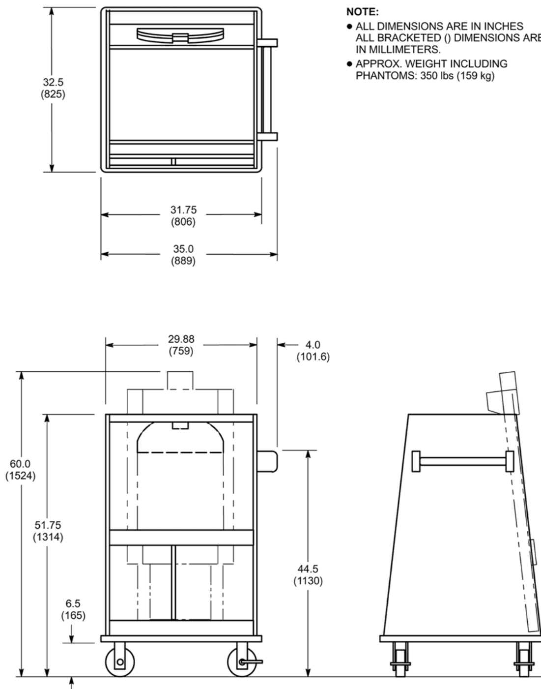
Illustration 3-15: SPT Phantom Set Shipping/Storage Cart
