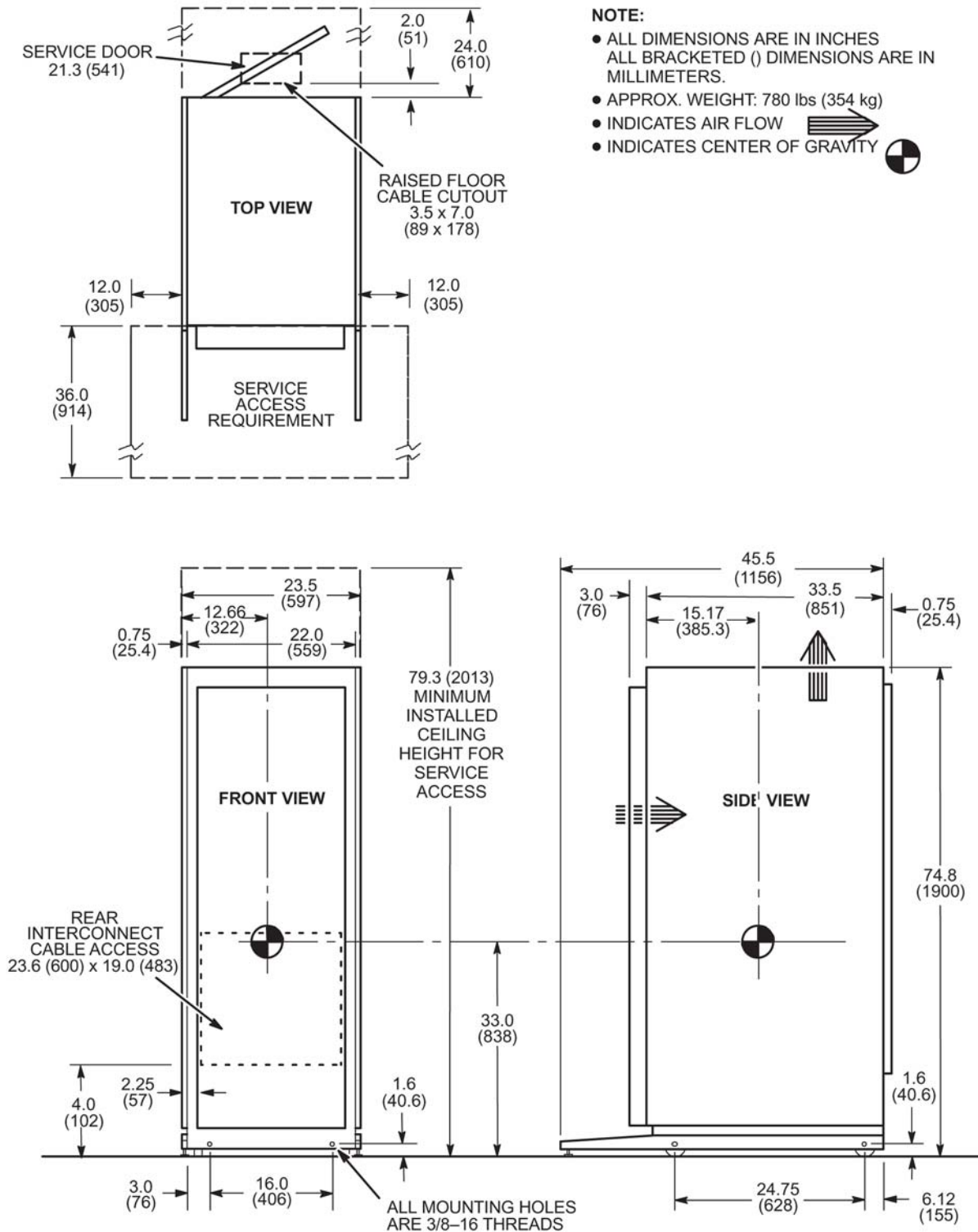
Illustration 3-42: 1.5T RFS Cabinet
