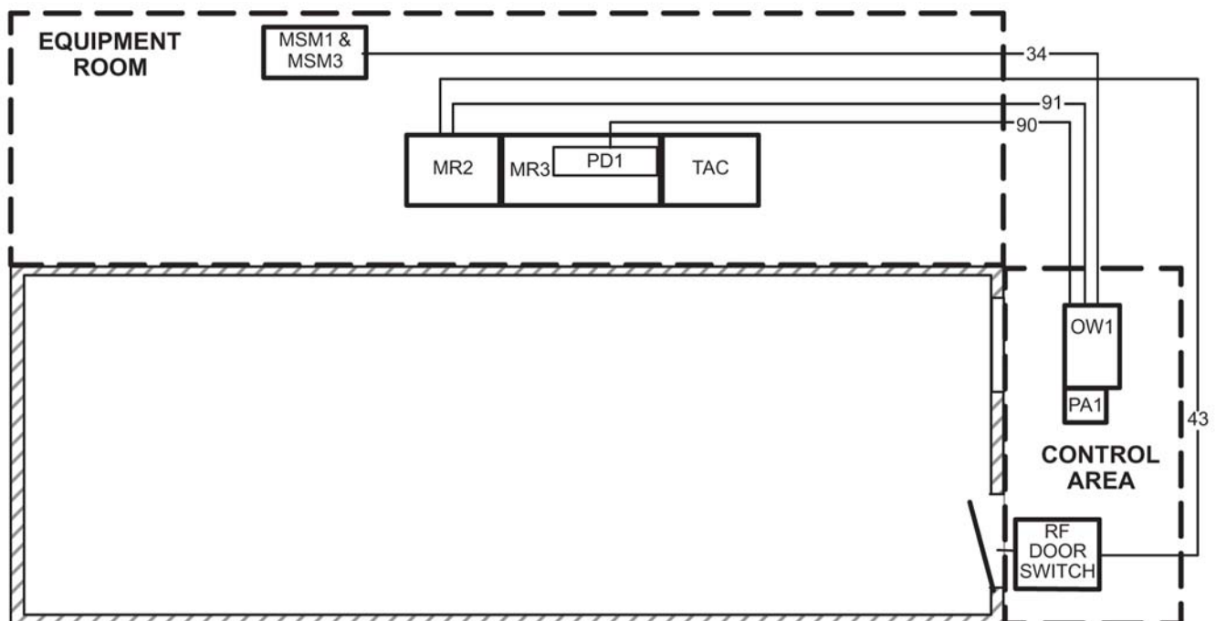
Illustration 7-18: System L5 Interconnects Diagram
