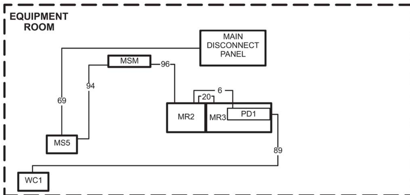
Illustration 7-14: System L3 Interconnects Diagram
