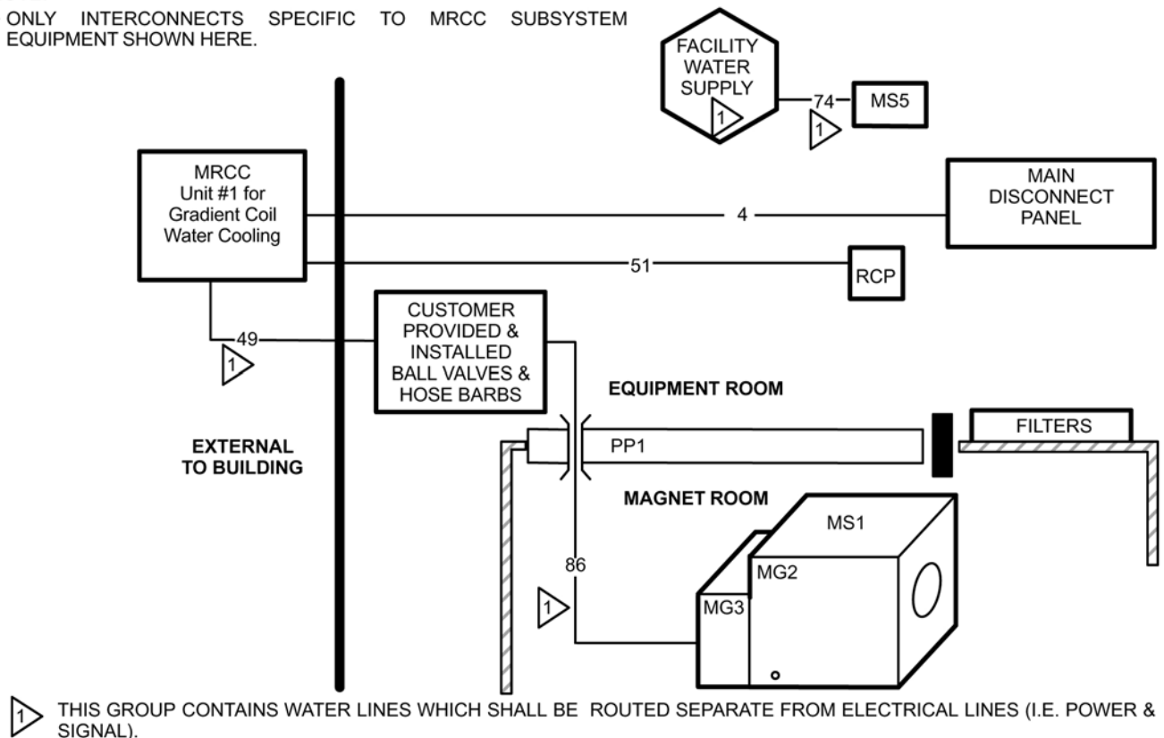
Illustration 7-27: 1 MRCC Unit Located Outdoor & RCP Subsystem Group Interconnect Diagram
